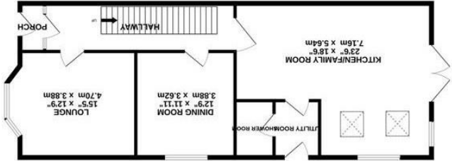
GROUND FLOOR 921 sq.ft. (85.5 sq.m.) approx.
